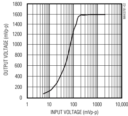
DIFFERENTIAL OUTPUT VOLTAGE vs. DIFFERENTIAL INPUT VOLTAGE
